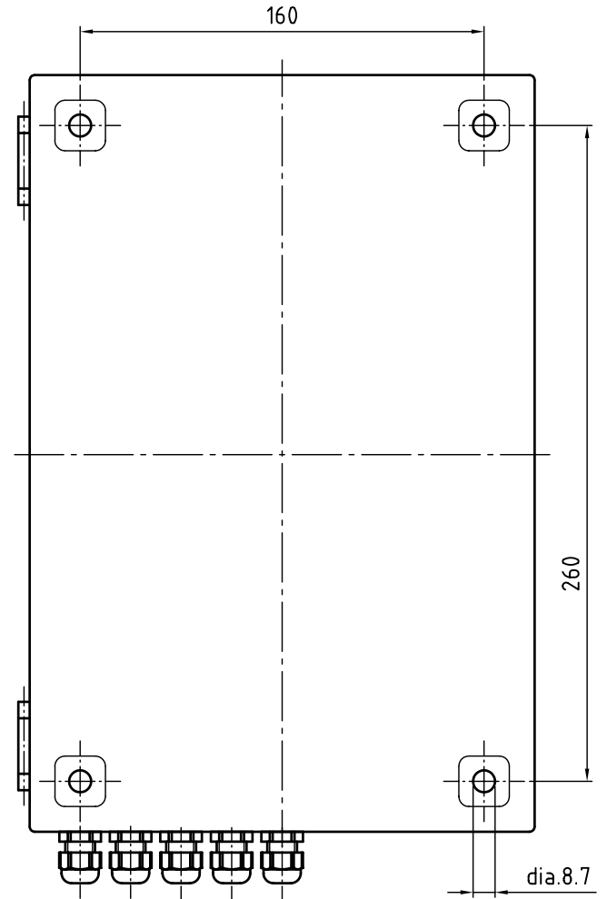
drilling template for mounting holes
